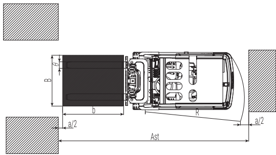
Ast=X+R+b+a b=Load Length a=Clearance(200mm)
