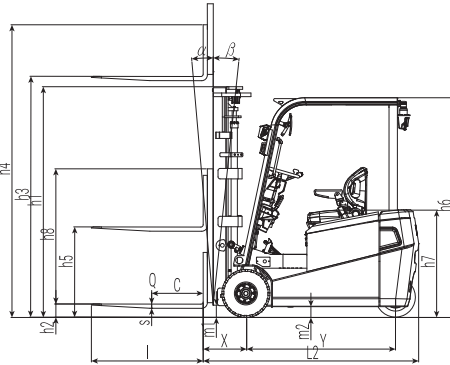
h5 = Free Lift of Duplex FFL & Triplex FFL Mast
